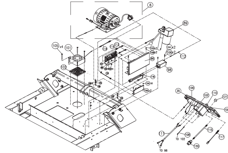
Detail View of Electrical Components
