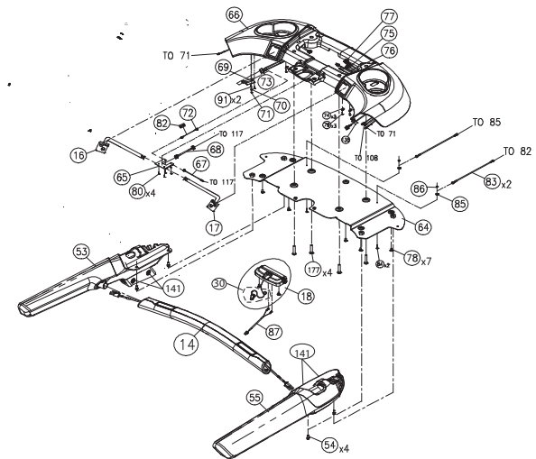
Detail view of Console Base
