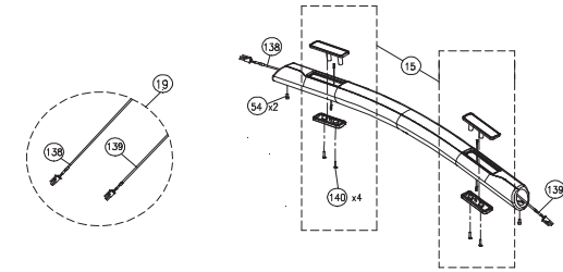
Detail view of Crossbar
