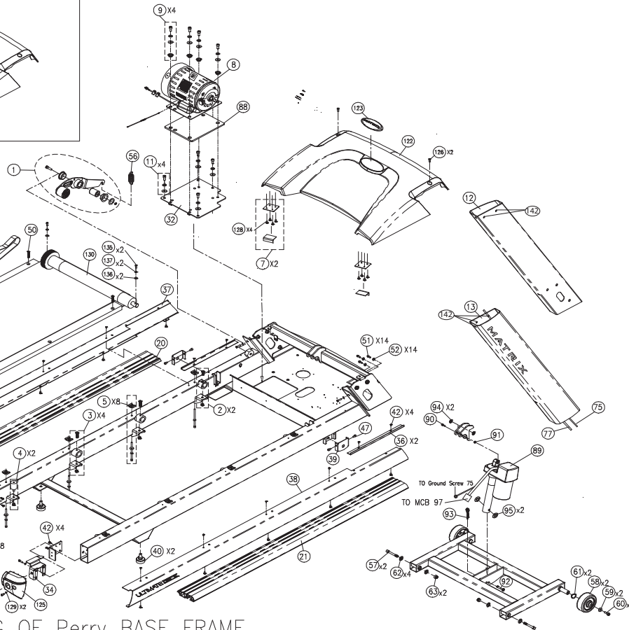
SERVICE DRAWING OF Perry BASE FRAME
