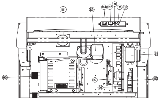
Top View of Electrical Components
